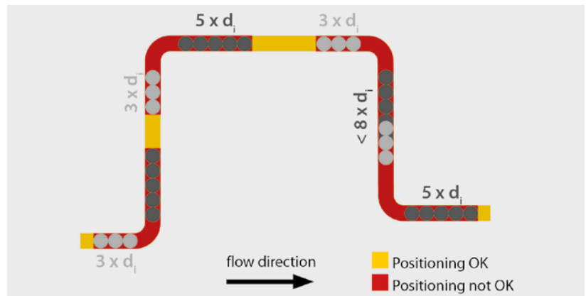
It is advisable to mount the sensor only in the yellow areas.
