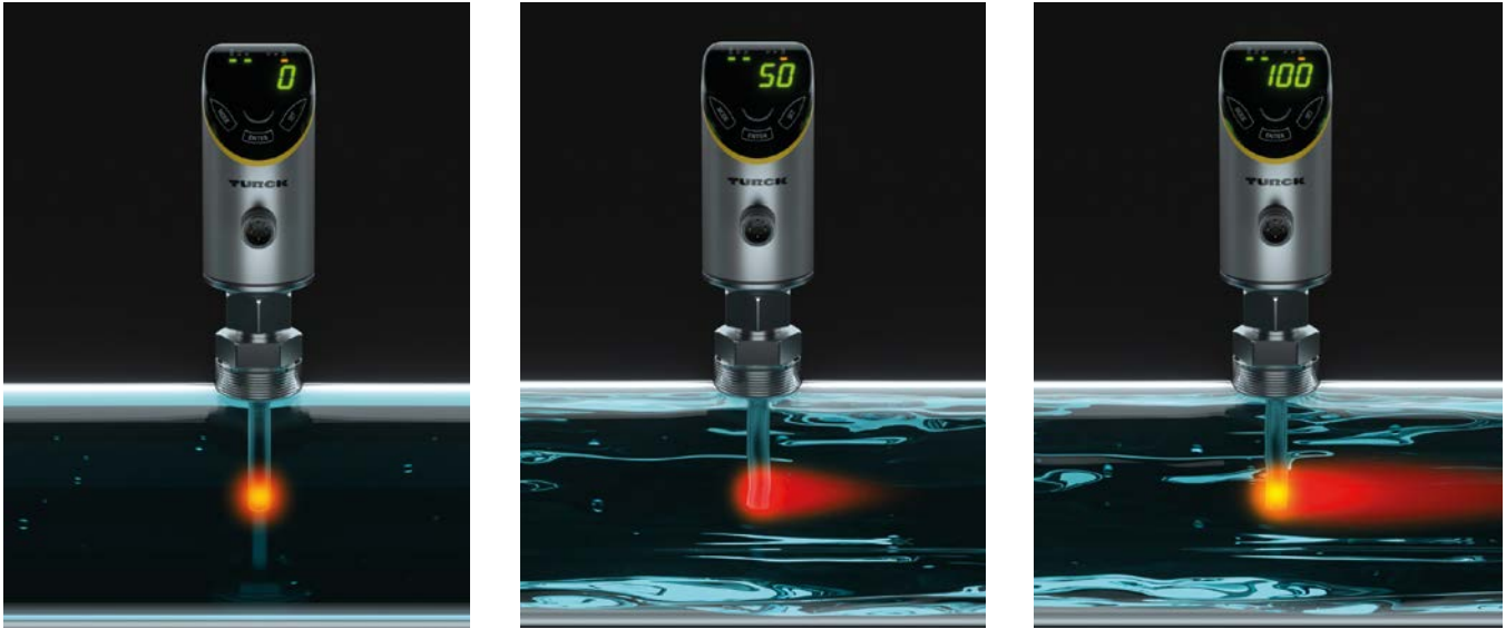
The probe of a calorimetric flow sensor is heated on one side. Two sensors inside the probe determine the temperatures on both sides. The temperature difference becomes smaller the faster the medium flows.
