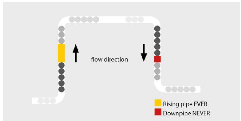
In vertical lines, the installation should be carried out in risers, since the compression of the medium there ensures a homogeneous flow pattern.
