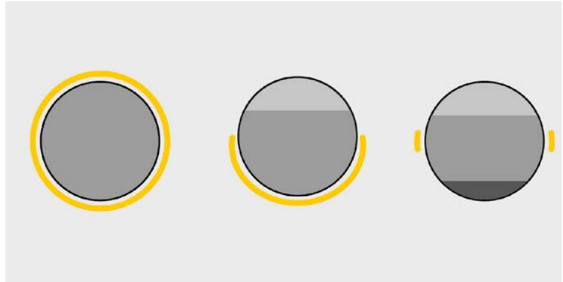
The yellow areas indicate good sensor positions for different pipe conditions. Air pockets and deposits reduce the number of possible positions for the flow sensor.
