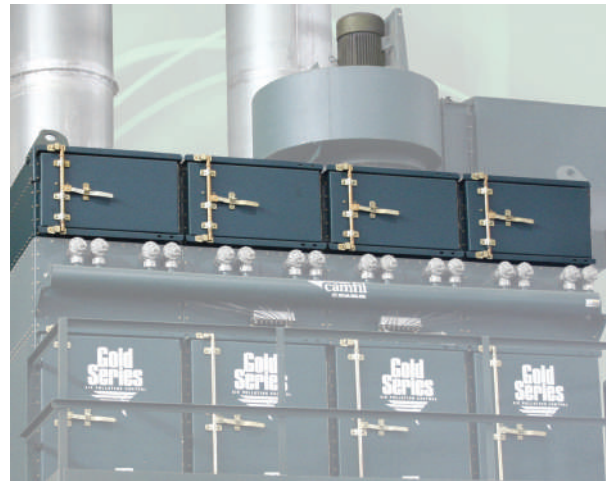
This space-saving after-filter module is integrated on top of the fume collector. It provides backup protection in a recirculating fume collection system.
